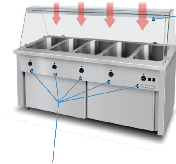
Her küvette ayrı termostatlı, ısı kontrollü Separate thermostat control for each bowl
